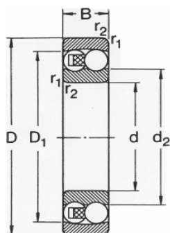
CYLINDRICAL BORE
